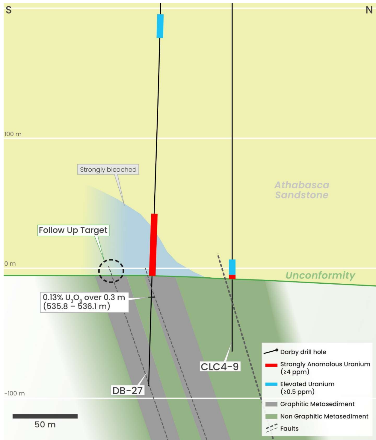
Figure 3 – Cross Section Through Delta Trend Drill Holes DB-27 and CLC4-9
