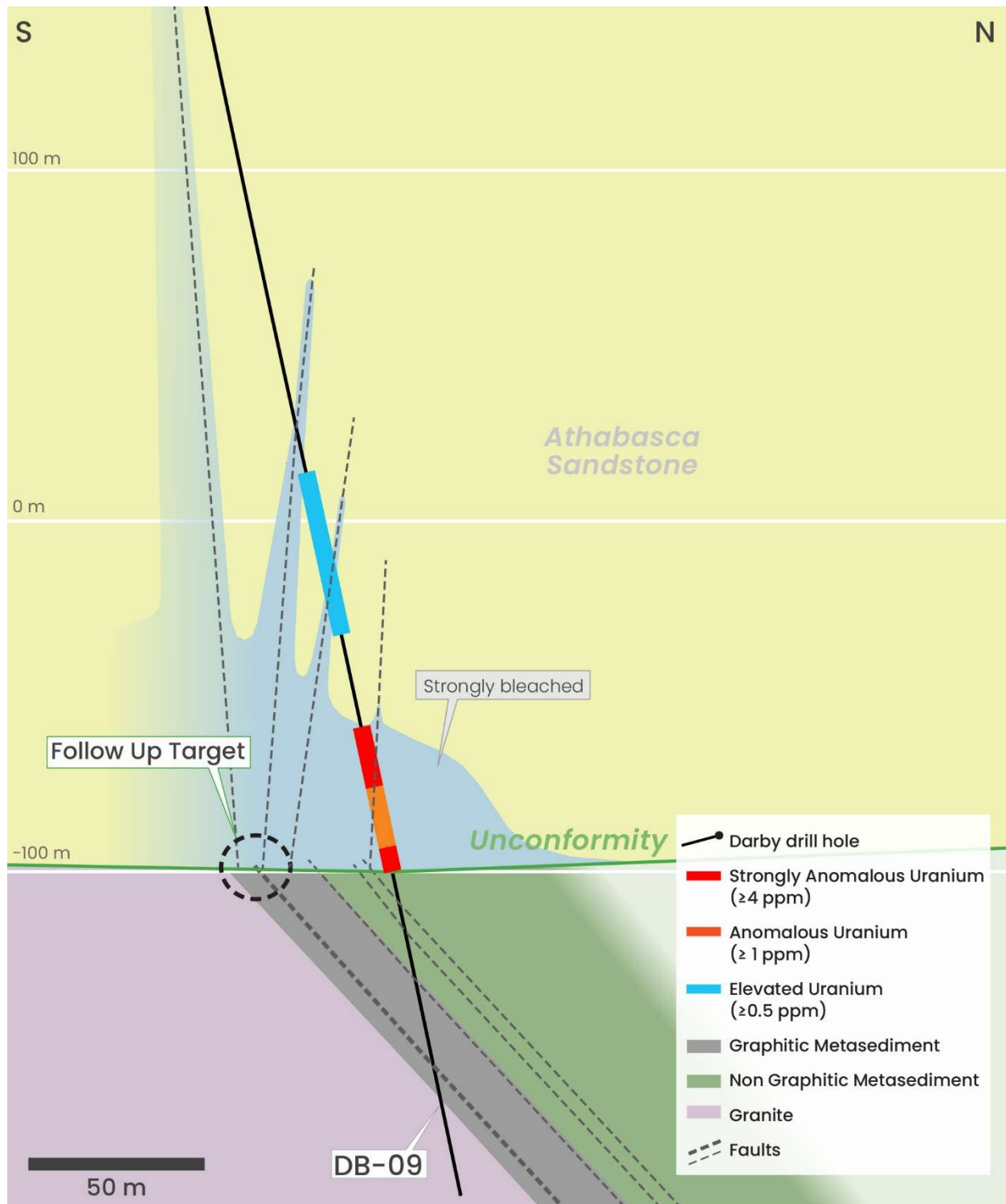
Figure 4 – Cross Section Through Charlie Trend Drill Hole DB-09
